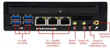
LPC-480G4M Front View
