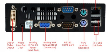
LPC-480G4M Rear View
